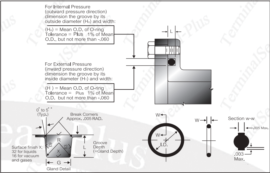
Design-For O-Ring Face Seal Glands
