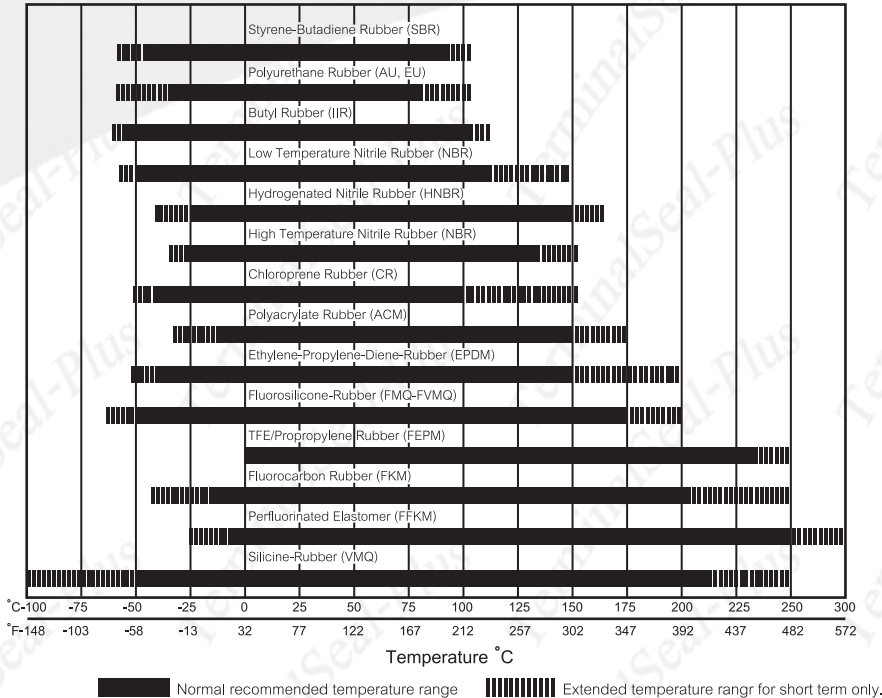
Temperature Range for Common Elastomeric Materials
