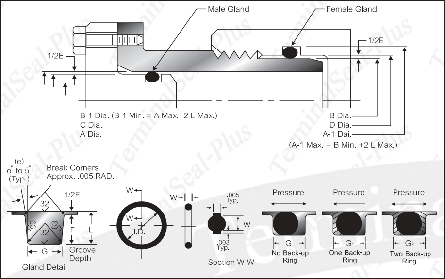
Design-For Industrial O-Ring Static Seal Glands
